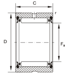
RNA 49..2RS
